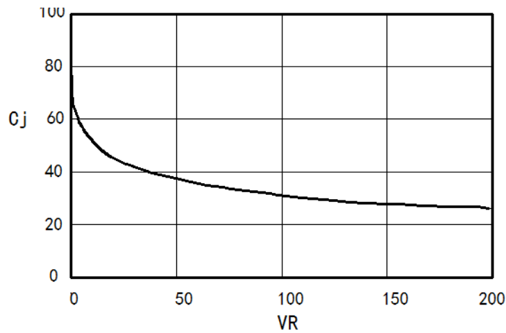
FIGURE 5. JUNCTION CAPACITANCE vs REVERSE VOLTAGE
