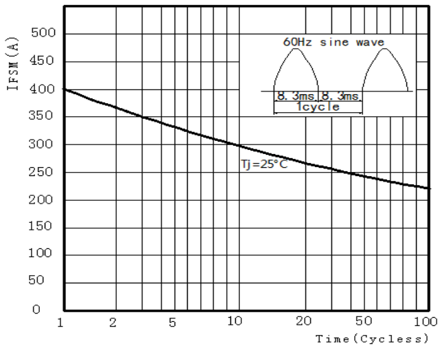
FIGURE 3. Peak Surge Forward Capability
