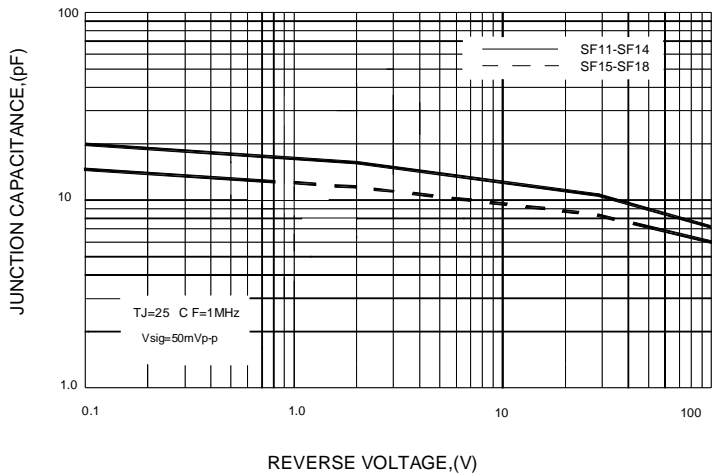
FIG.5-TYPICAL JUNCTION CAPACITANCE
