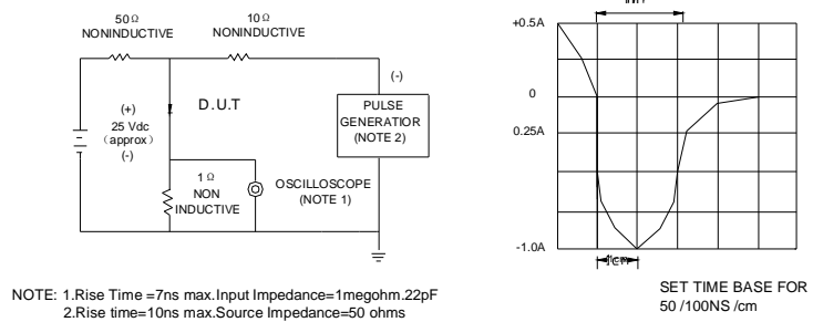
FIG.6-TEST CIRCUIT DIAGRAM AND REVERSE RECOVERY TIME CHARACTERISTIC
