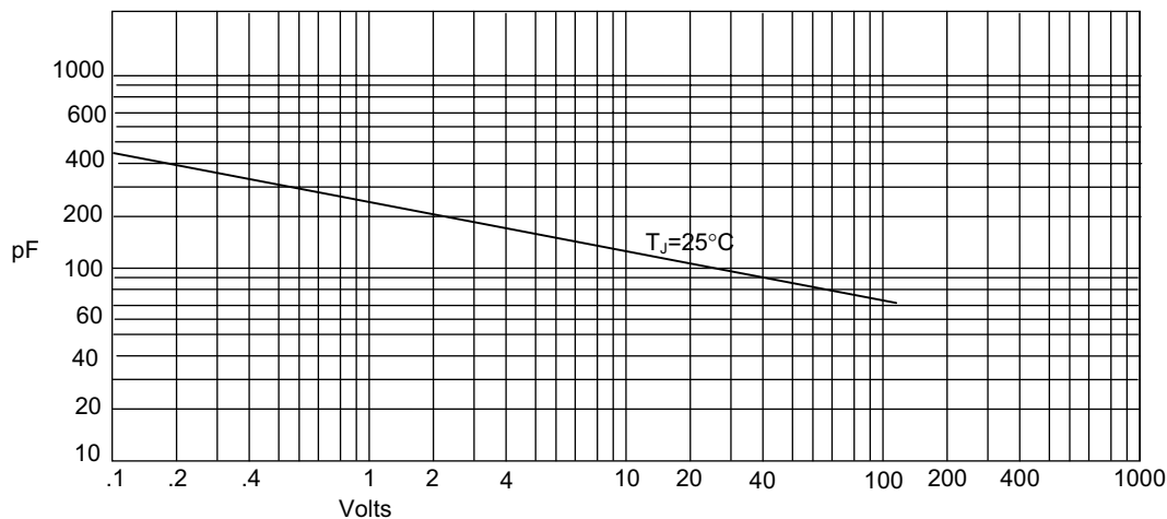
Figure 3 Junction Capacitance
