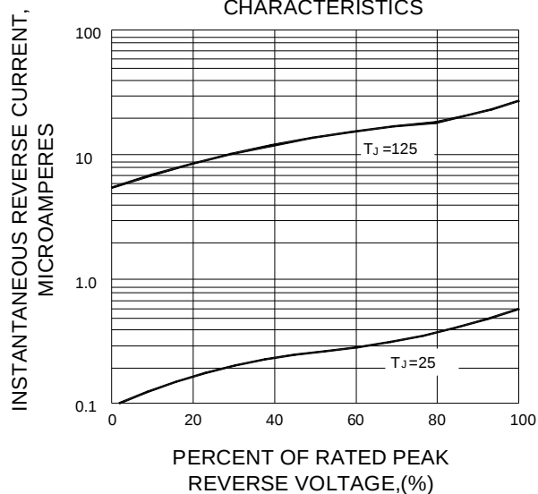
F1G.4-TYPICAL REVERSE CHARACTERISTICS
